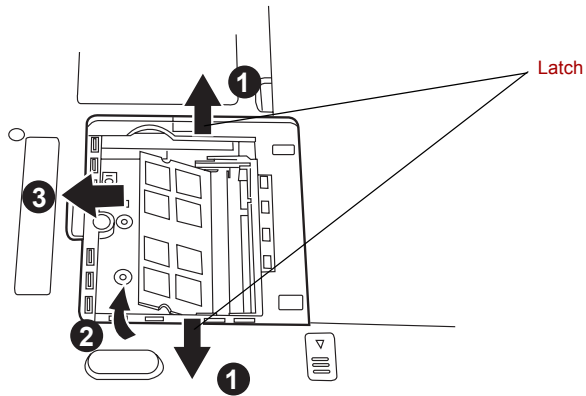
Removing the memory module
